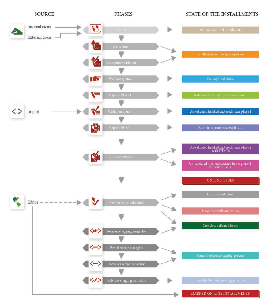
Figure 1 RIS registration, validation and normalization process
